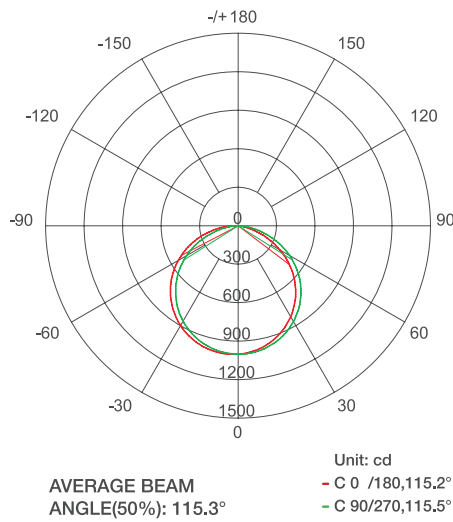
Beam Angle Diagram
